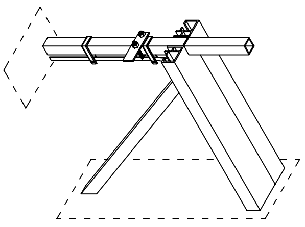
DETAIL A-3: TOP-TRACK ASSEMBLY
