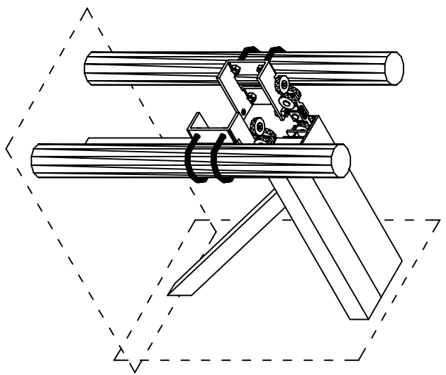
DETAIL A-3: TOP-TRACK ASSEMBLY
